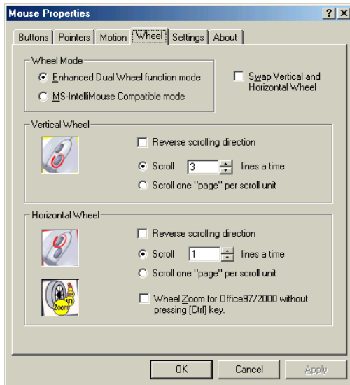
Figure 9: 'Wheel' tab
