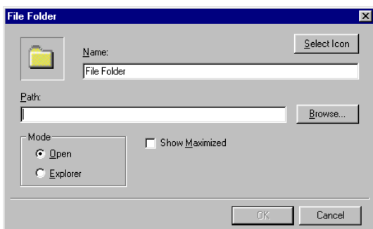
Figure 14: File Folder
