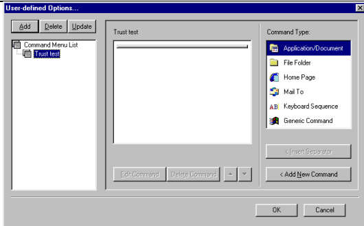
Figure 12: User options
