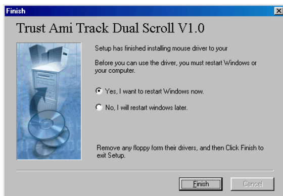
Figure 5: Installation completed
