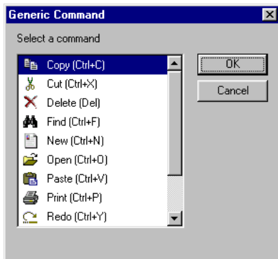
Figure 18: Generic Command
