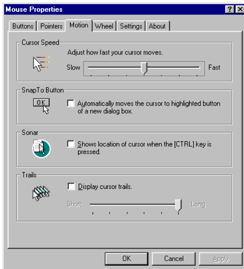
Figure 8: 'Motion' tab
