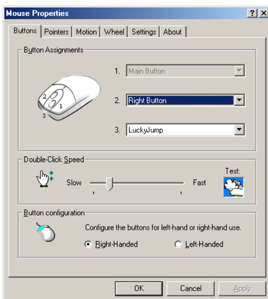
Figure 7: 'Buttons' tab
