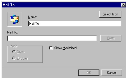
Figure 16: Mail To
