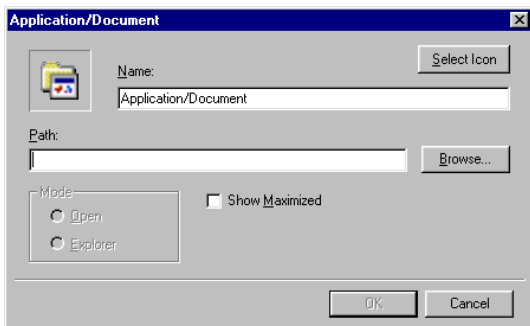
Figure 13: Application/Document
