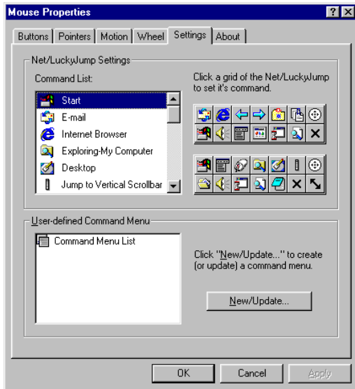
Figure 10: 'Settings' tab
