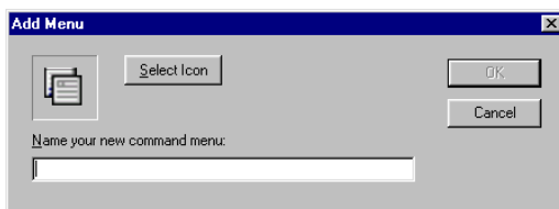
Figure 11: Add menu
