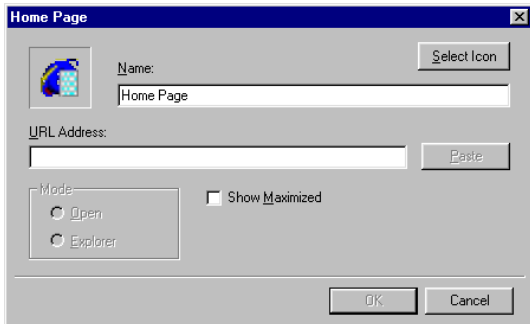
Figure 15: Home Page
