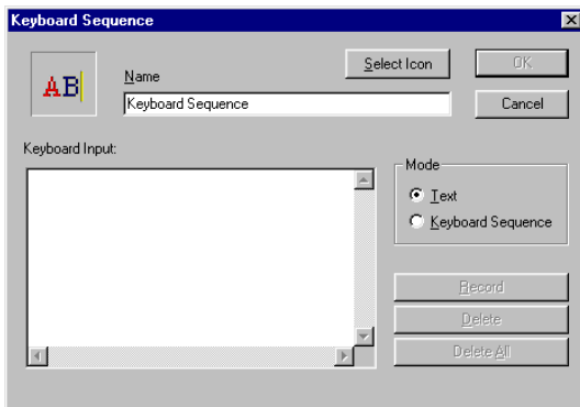
Figure 17: Keyboard Sequence
